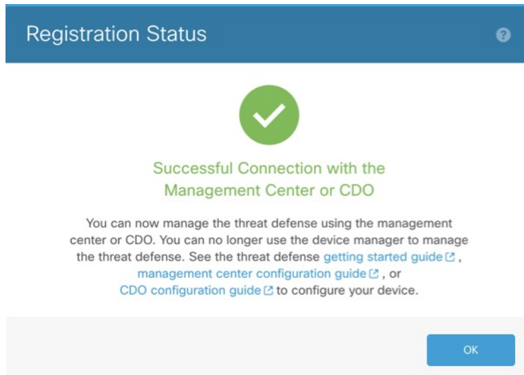
Figure 2: Successful Connection
