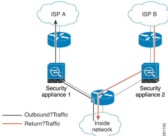
Figure 1: Asymmetric Routing
