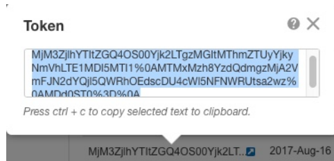
Figure 10: Copy Token
