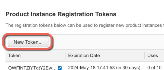
Figure 12: New Token
