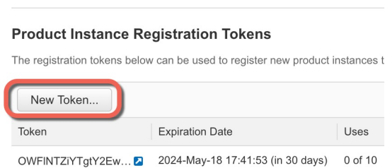
Figure 2: New Token
