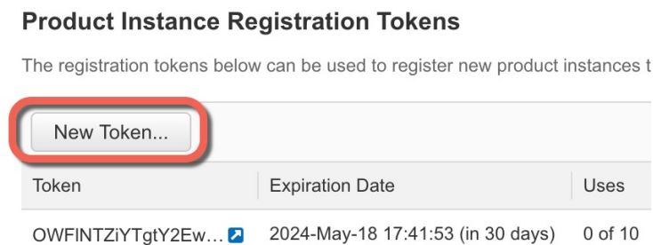
Figure 7: New Token
