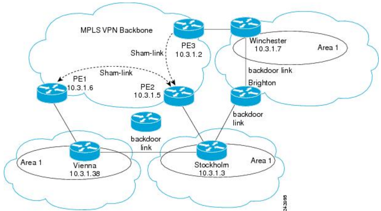
Figure 20: Sham Link Between PE Routers to Connected OSPF Client Sites
