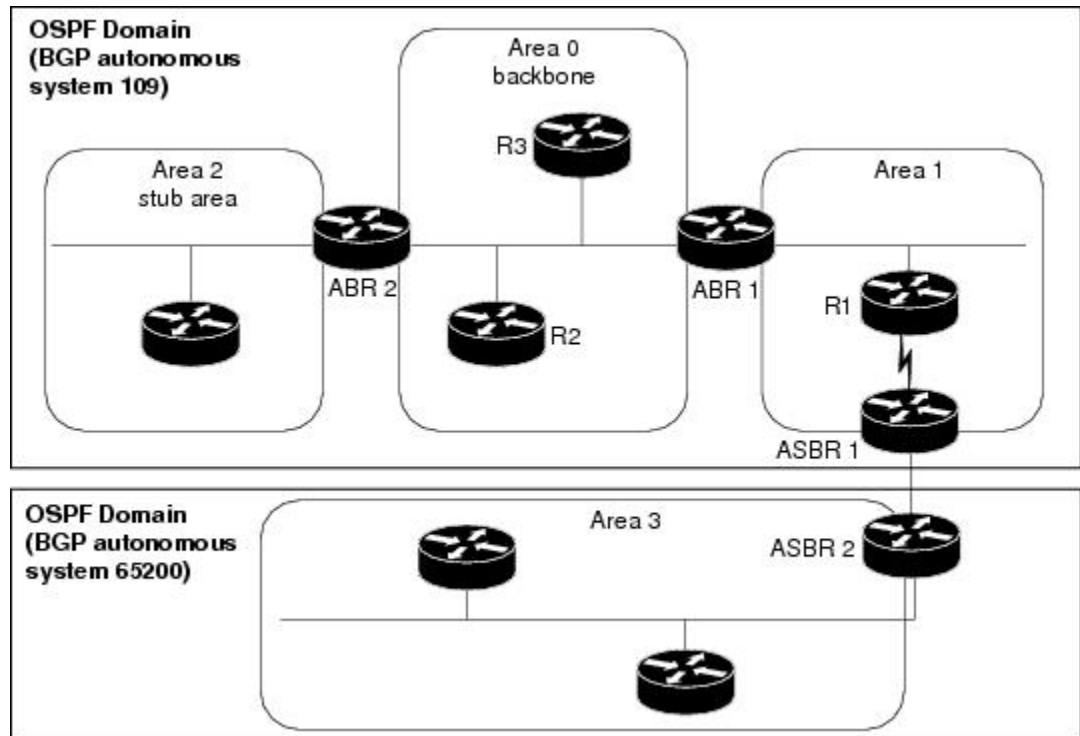
Figure 17: OSPF Routing Components
