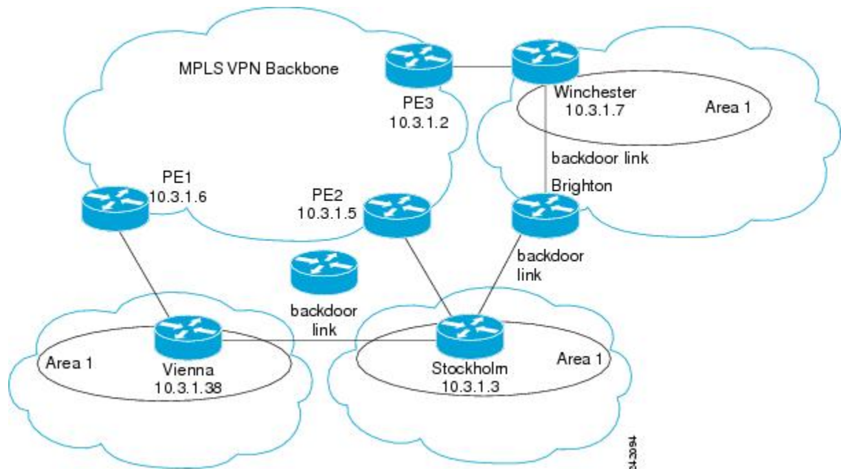
Figure 19: Backdoor Paths Between OSPF Client Sites
