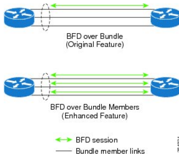
Figure 13: BFD Sessions in Original BFD Over Bundles and Enhanced BFD Over Bundle Member Links Architectures
