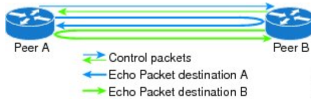
Figure 12: BFD Asynchronous Mode With Echo Packets
