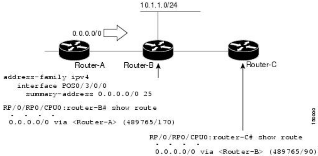
Figure 14: Floating Summary Route Is Applied to Router-B
