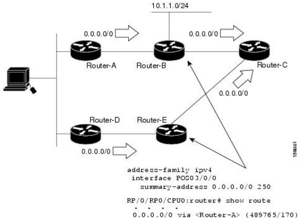
Figure 15: Floating Summary Route Applied for Dual-Homed Remotes
