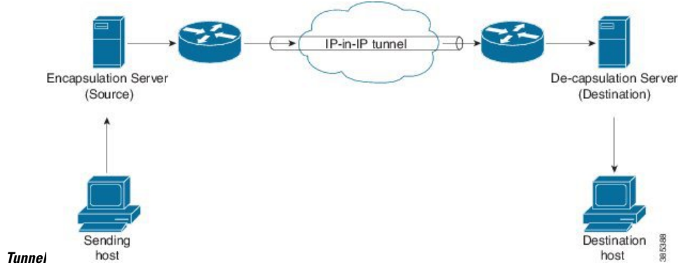
Figure 6: Basic Encapsulation and De-capsulation with an IP-in-IP
