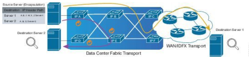
Figure 7: IP-in-IP De-capsulation through a Data Center Network
