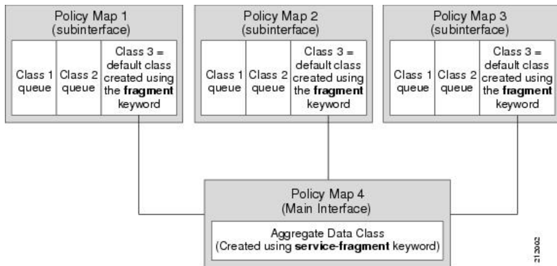
Figure 2: Physical Interface with Policy-Maps—Using Fragments
