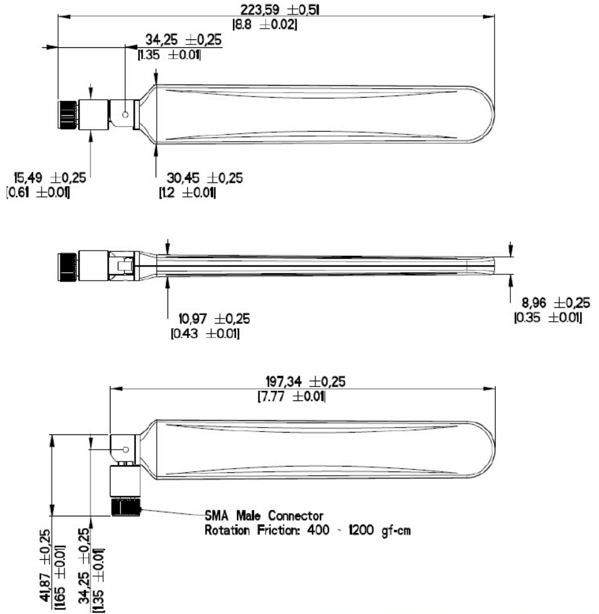
Figure 2: Mechanical Drawing
