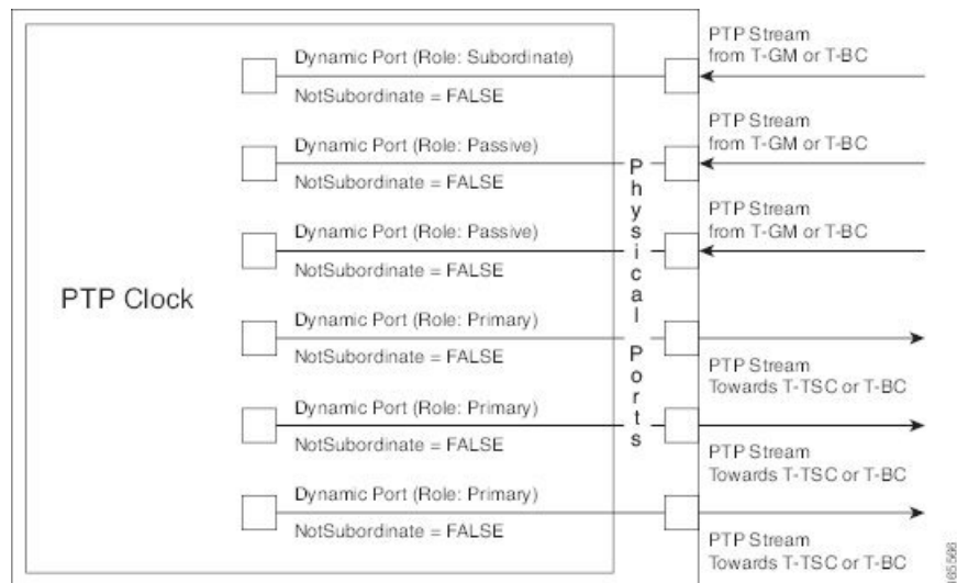
Figure 4: Boundary Clock
