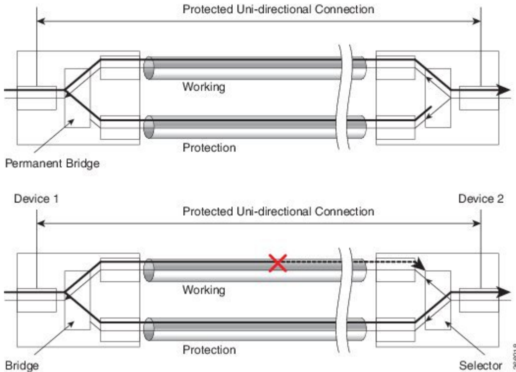
Figure 2: Unidirectional MSP 1+1
