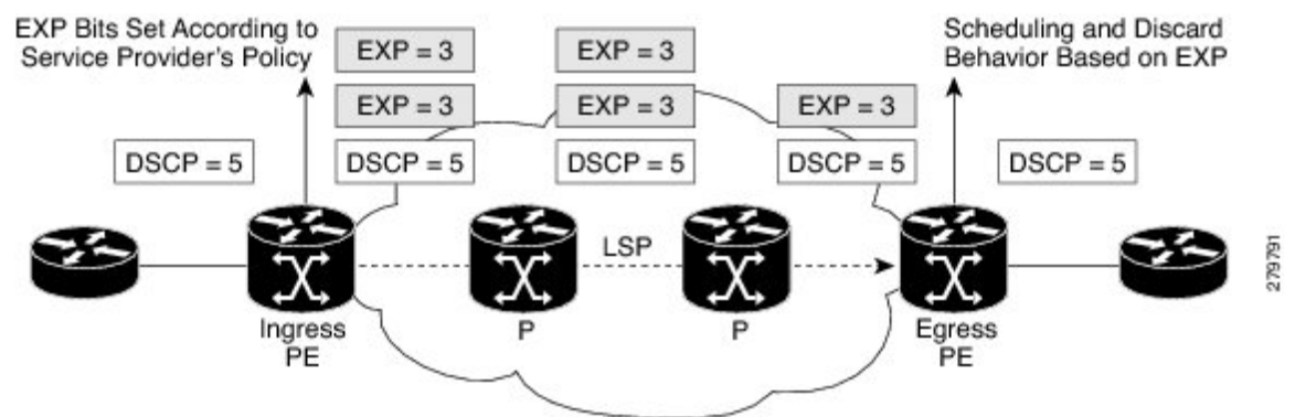
Figure 4: Pipe Mode
