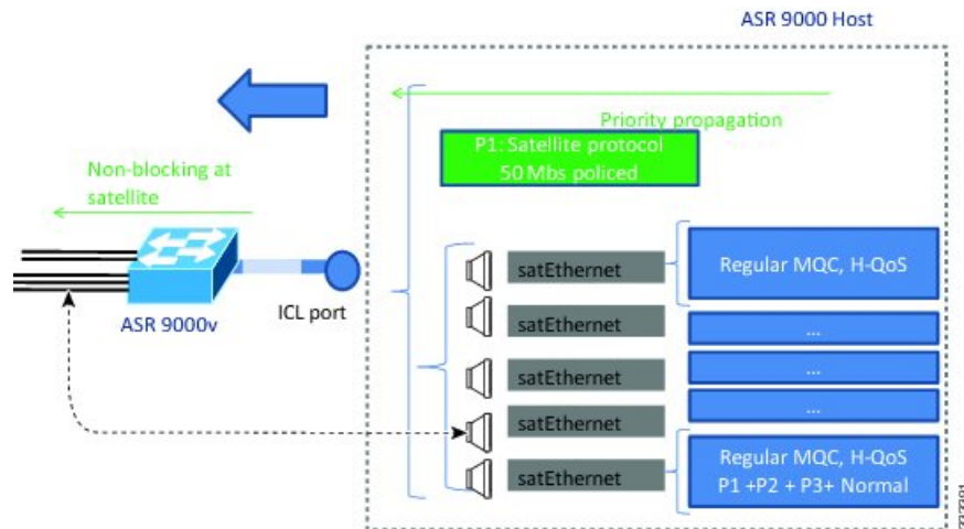
Figure 2: AutoQoS, host to satellite
