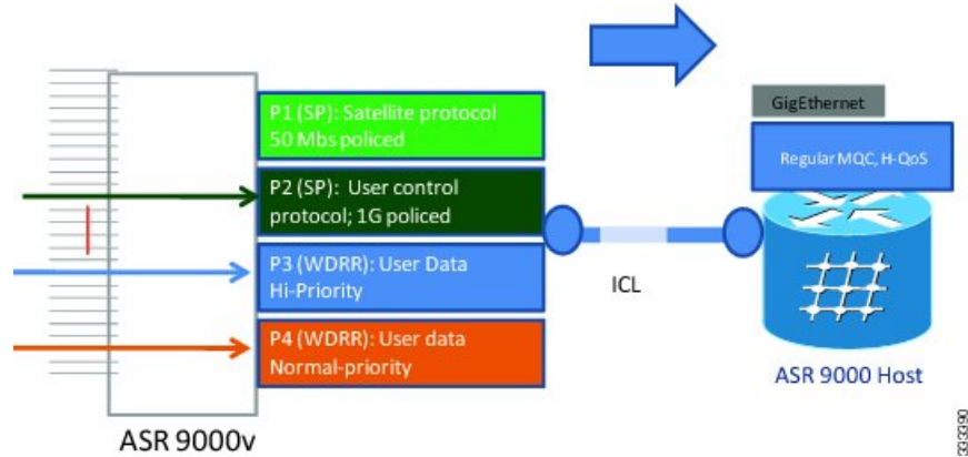
Figure 1: AutoQoS, Cisco ASR 9000v satellite to host
