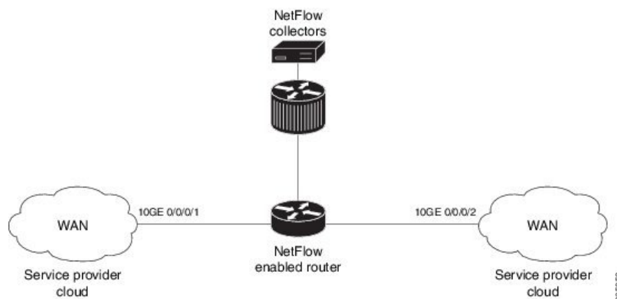
Figure 3: SP-PE Topology
