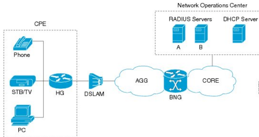
Figure 1: BNG Architecture
