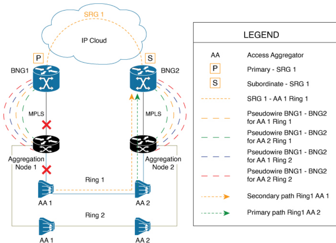
Figure 38: Link Failure Scenarios in BNG PWHE topology with SRG
