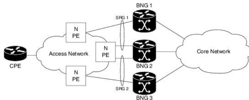
Figure 26: BNG Subscriber Redundancy Group
