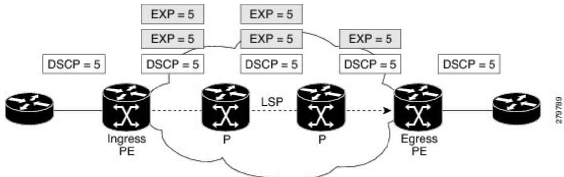
Figure 10: Uniform Mode
