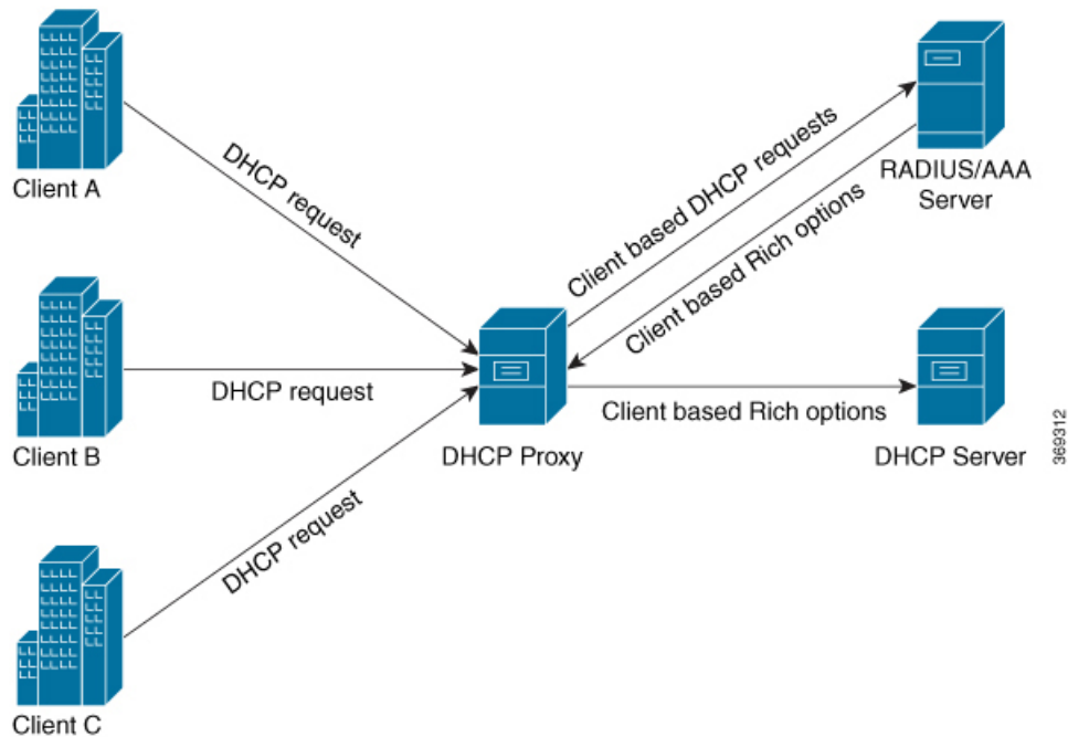
Figure 14: Flow of Rich Options From AAA Server to DHCP Proxy
