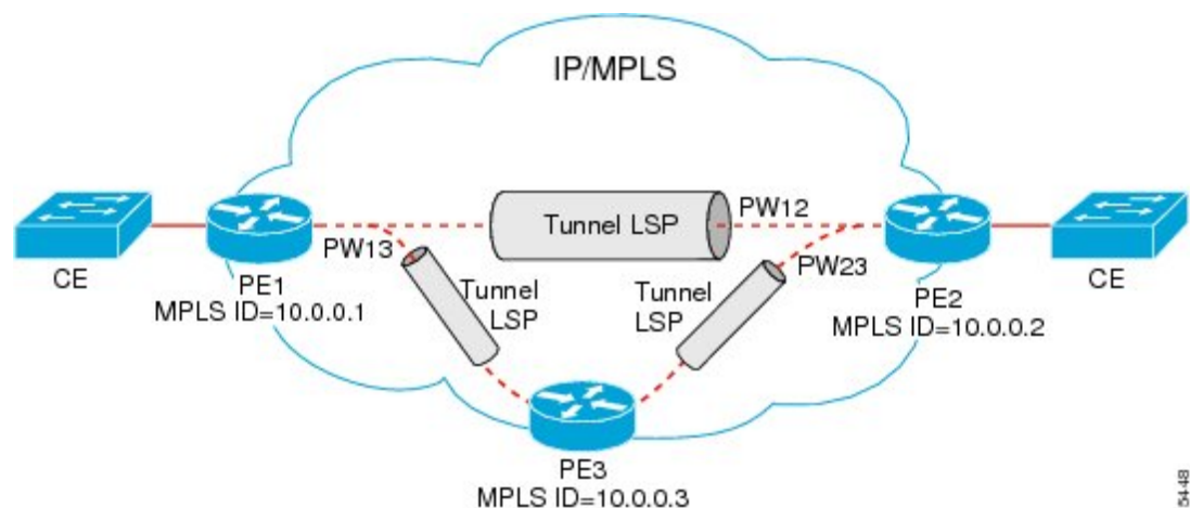
Figure 6: Typical VPLS Network Topology
