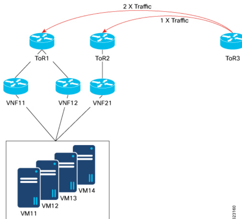
Figure 26: Proportional Multipath
