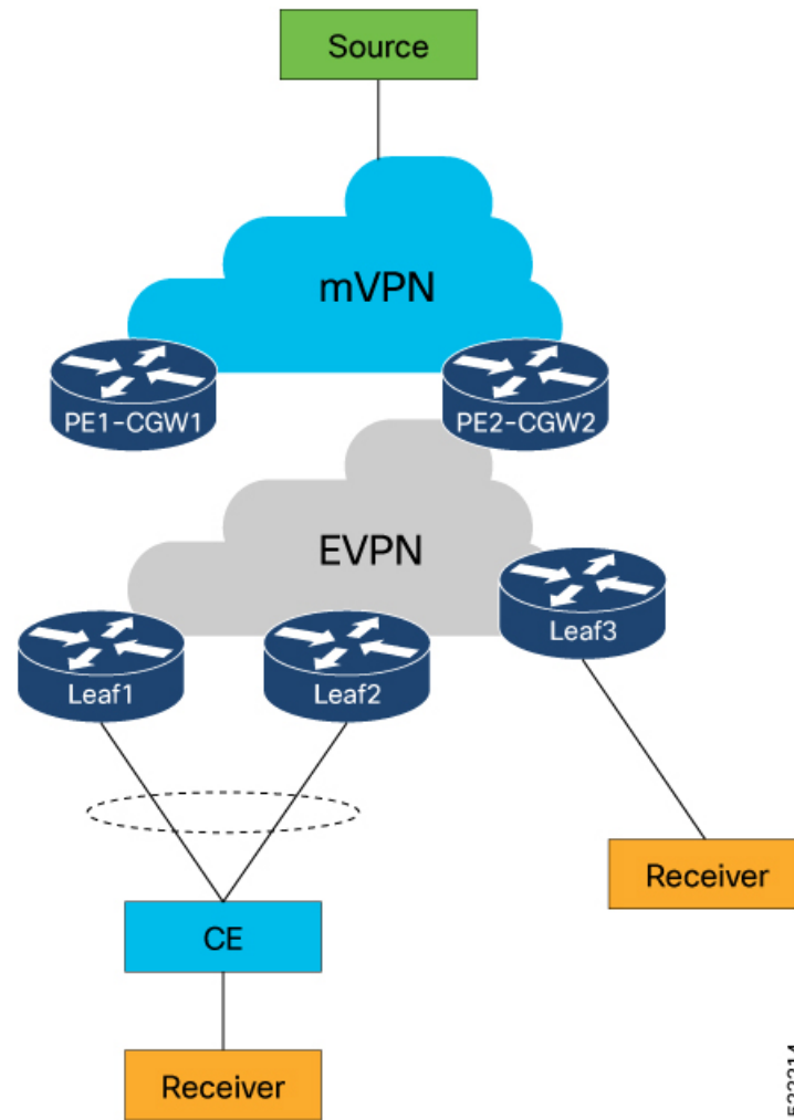
Figure 25: Topology
