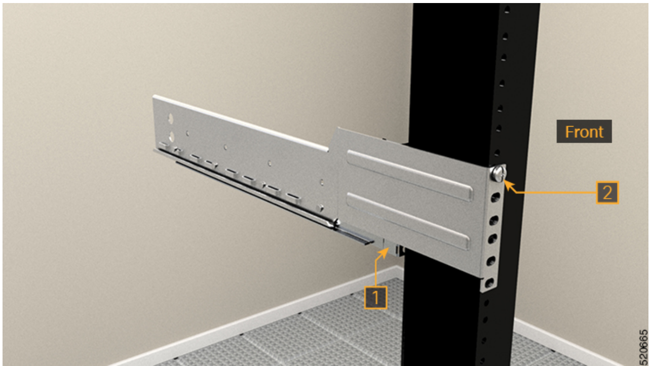
Figure 9: Two Post Slider Integration in the 19" Rack
