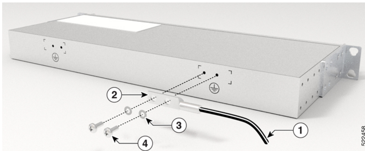
Figure 2: Grounding the Patch Panel
