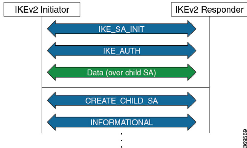
Figure 6: IKEv2 Exchanges
