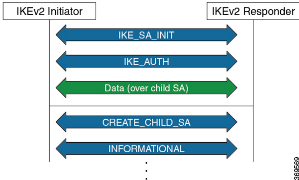
Figure 6: IKEv2 Exchanges
