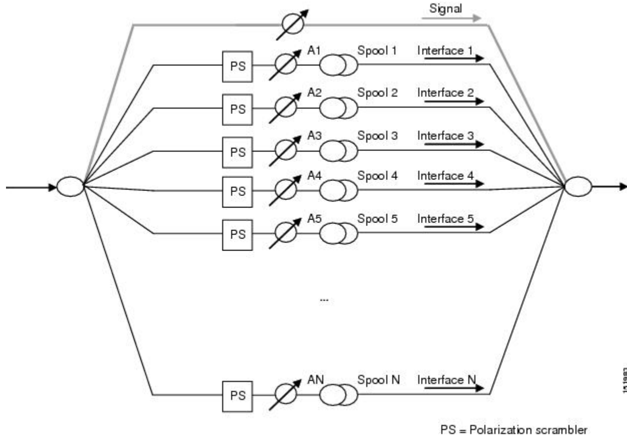
Figure 6: Generation Block for Gaussian Cross-Talk Measurement
