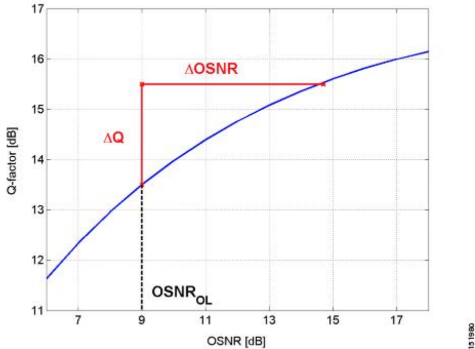
Figure 3: Q-Factor Curve
