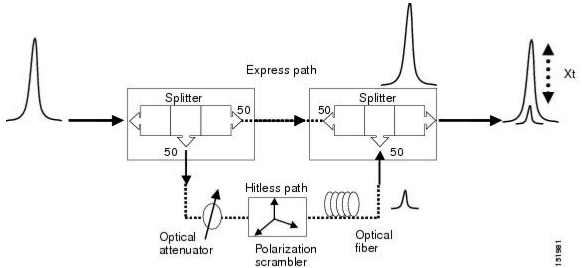
Figure 5: Block Diagram for Crosstalk Measure
