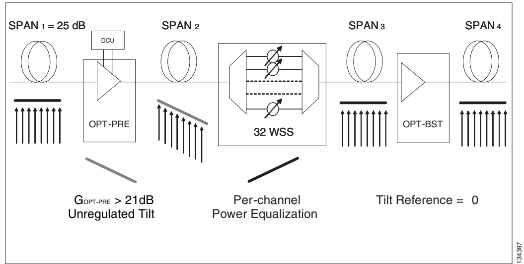
Figure 12-42 System Tilt Compensation With an ROADM Node
