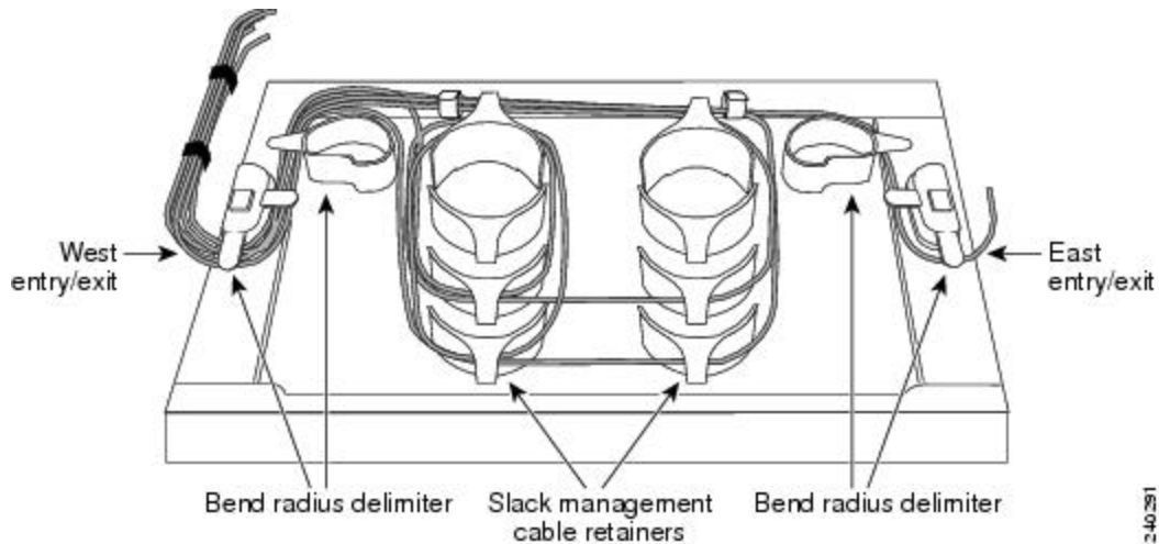
Figure 14: Fiber-Storage Tray
