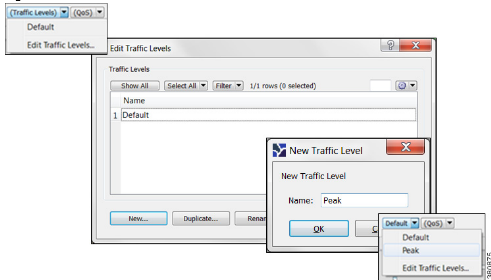
Figure 4-4 Create and Edit Traffic Levels
