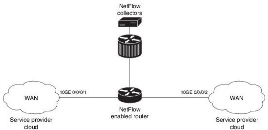
Figure 3: SP-PE Topology
