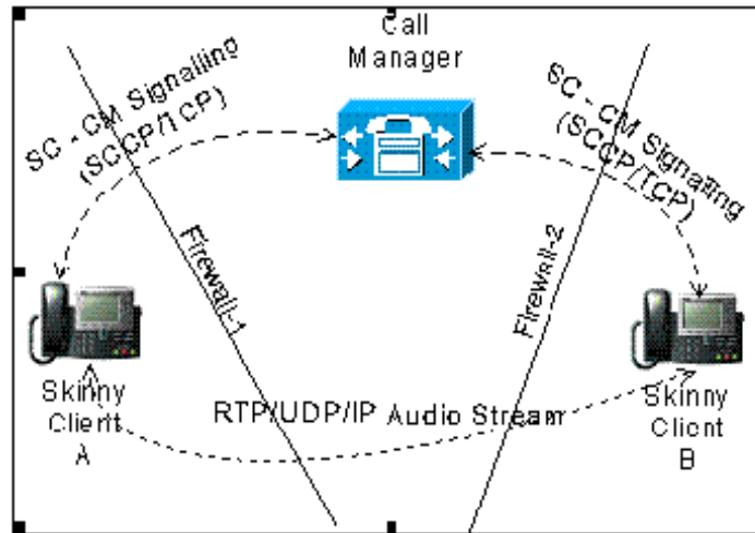
Figure 2 Skinny Client to Skinny Client Communication
