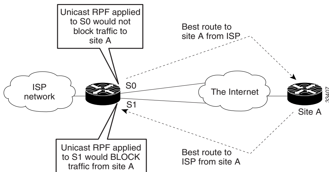
Figure 5 Unicast RPF Blocking Traffic in an Asymmetrical Routing Environment
