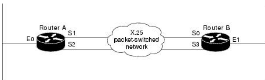
Figure 17: Parallel Serial Lines to an X.25 Network
