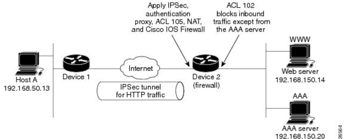
Figure 7 Authentication Proxy, IPsec, NAT, and CBAC Configuration Example
