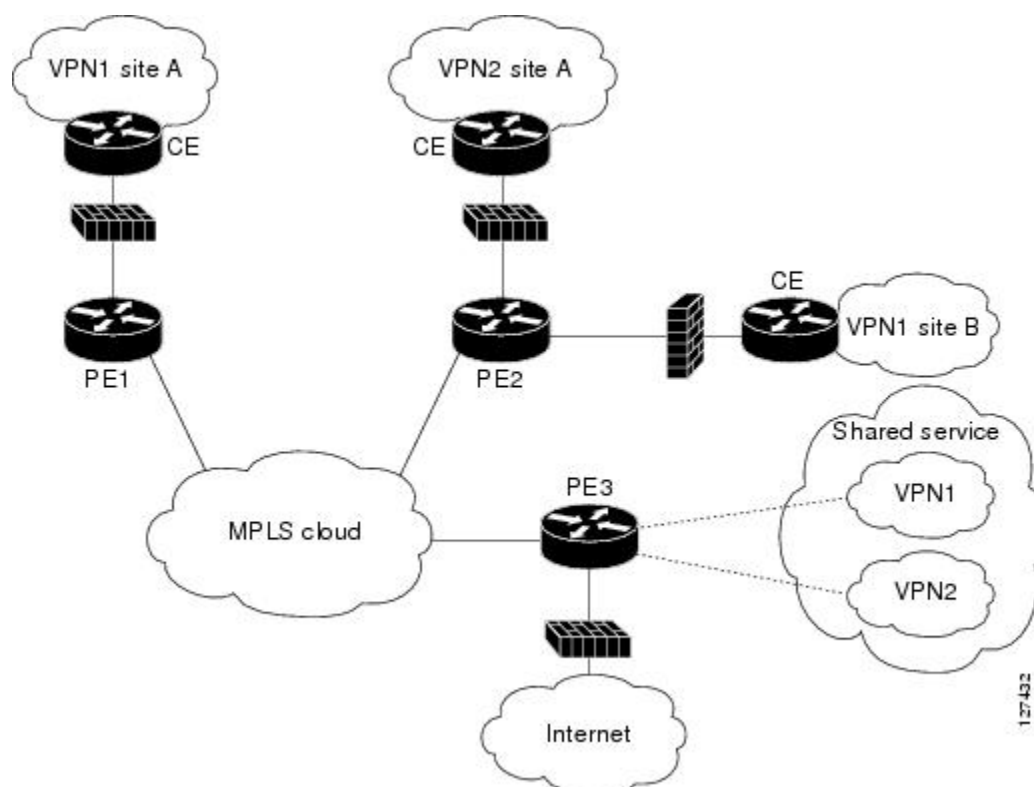
Figure 3 Distributed Network
