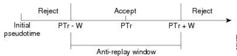
Figure 9 Antireplay Window
