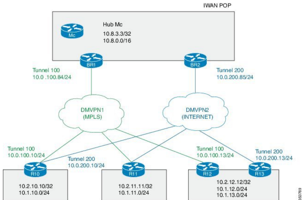
Figure 3: PFRv3 Topology
