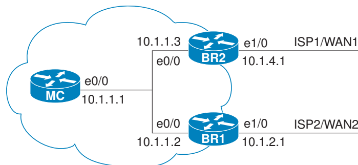
Figure 2 Network Diagram of OER Master Controller and Border Routers
