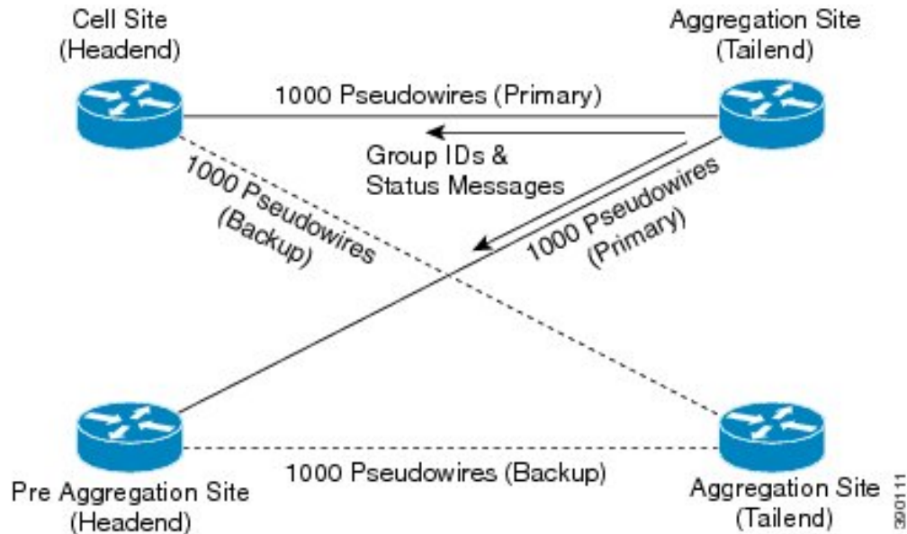
Figure 1: Primary and Backup Pseudowire Groups
