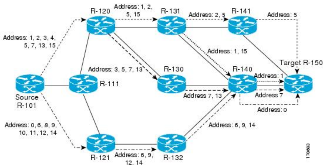
Figure 3: MPLS LSP Multipath Tree Trace Path Discovery in a Sample Network
