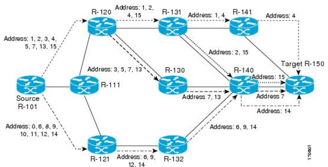
Figure 1: MPLS LSP Multipath Tree Trace Path Discovery in a Sample Network
