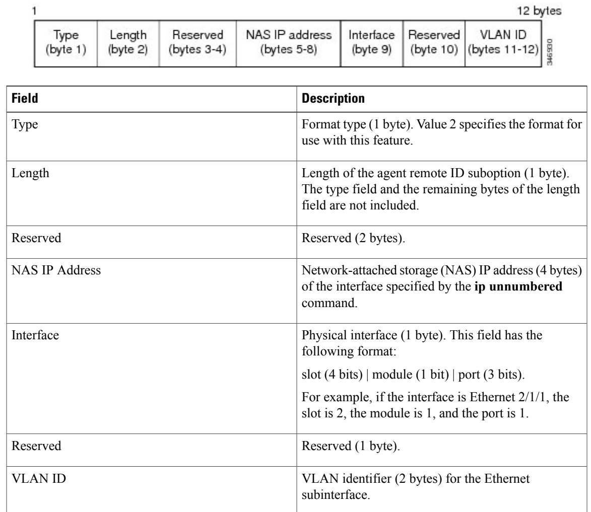
Figure 2: Format of the Agent Remote ID Suboption
