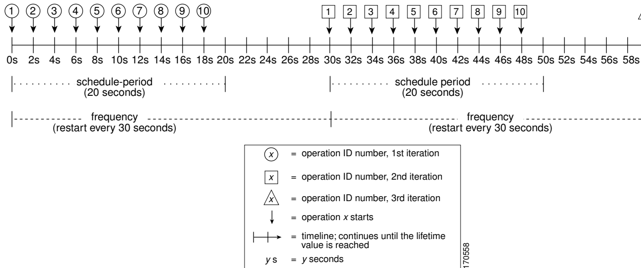
ip sla group schedule 2 1-10 schedule-period 20 frequency 30
