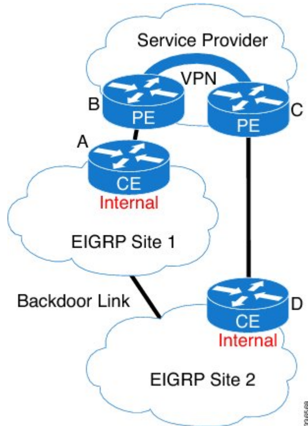
Figure 1: EIGRP 6PE/6VPE Functionality
