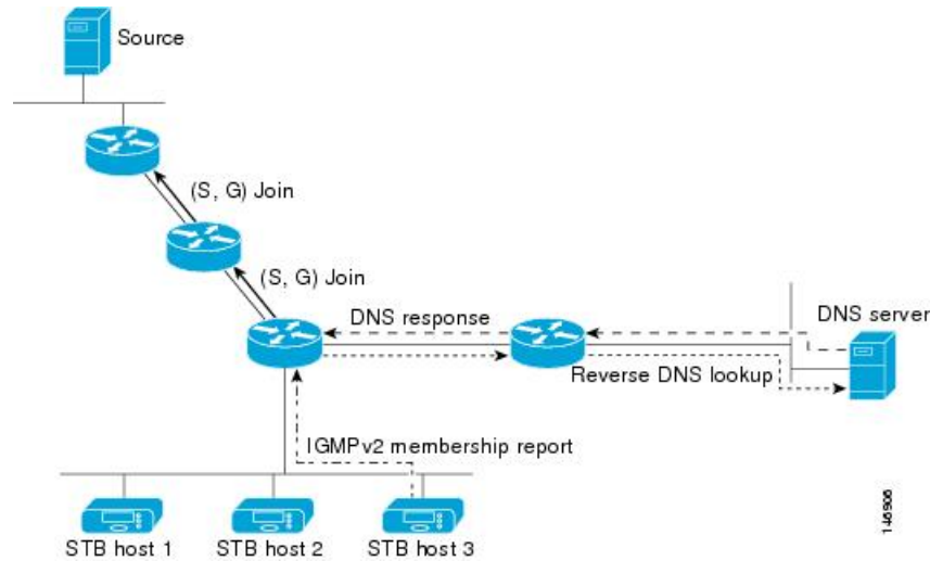
Figure 1: DNS-Based SSM-Mapping
