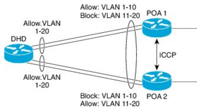
Figure 1: Active/Active Support
