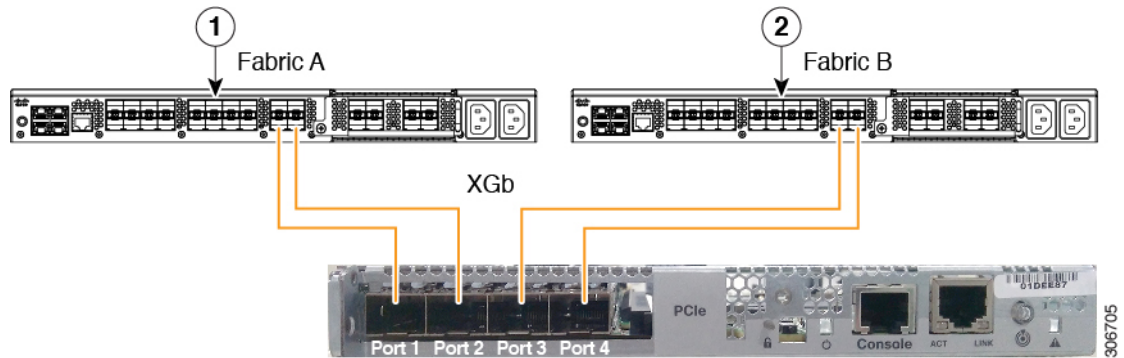
Figure 11: Direct Connect Cabling Configuration with Cisco VIC 1455
