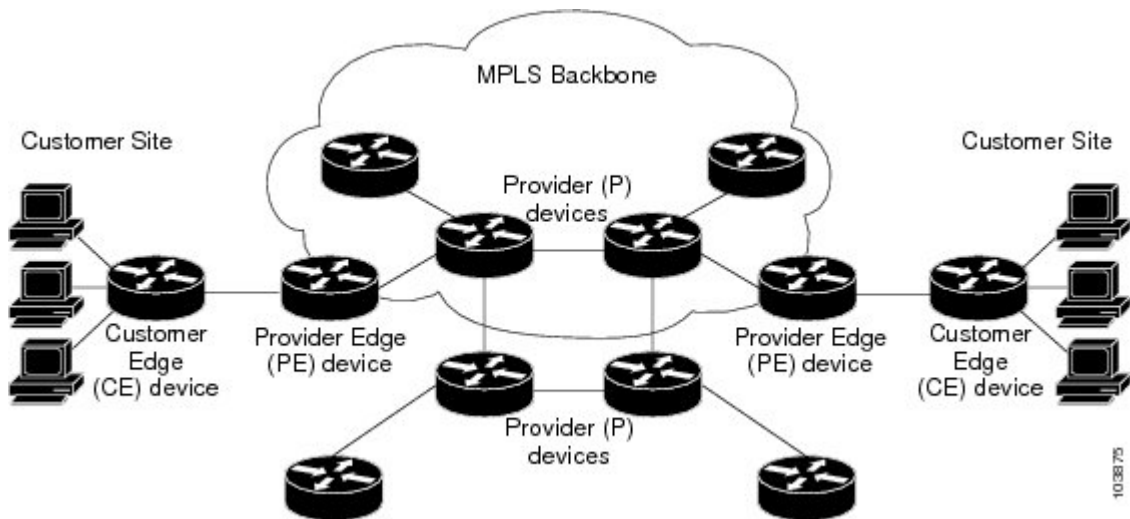
Figure 4: Basic MPLS Layer 3 VPN Terminology
