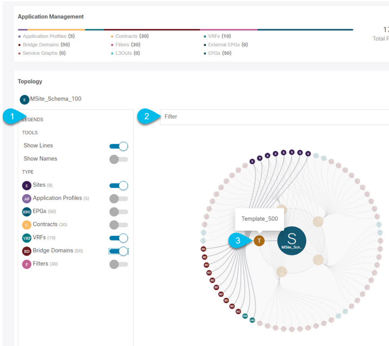
Figure 2: Deployment Visualizer
