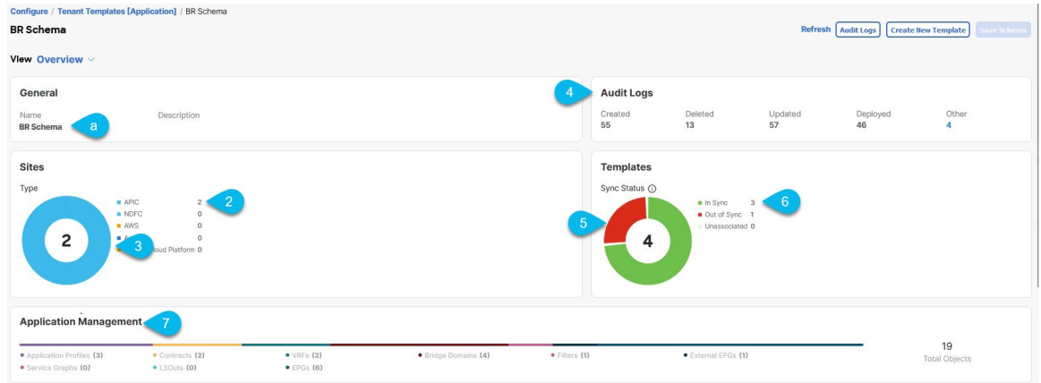
Figure 1: Schema Overview
