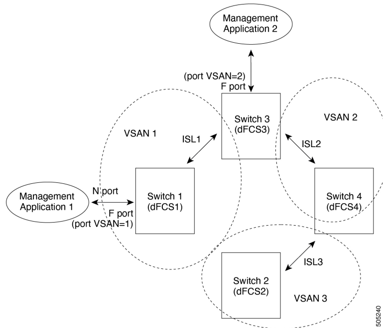
Figure 1: FCSs in a VSAN Environment
