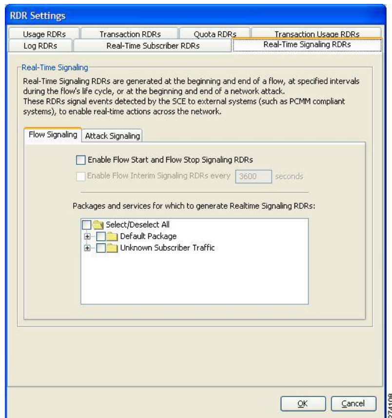
Figure 7: Real-Time Signaling RDRs Tab
