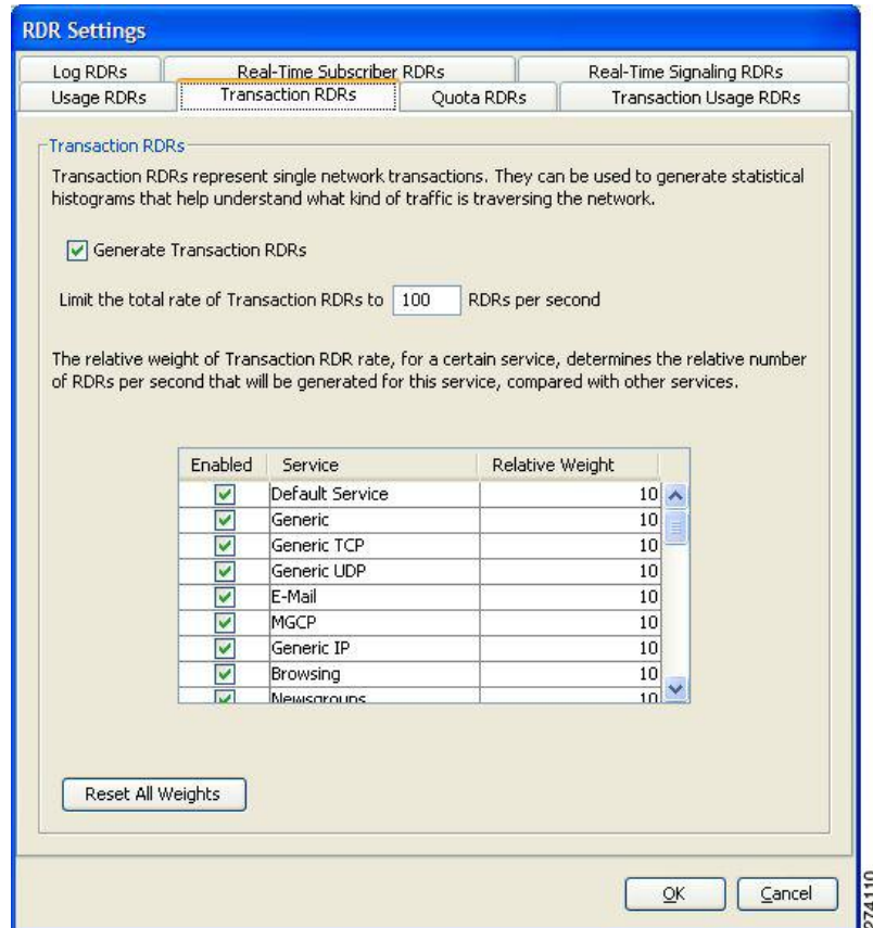
Figure 2: Transaction RDRs Tab
