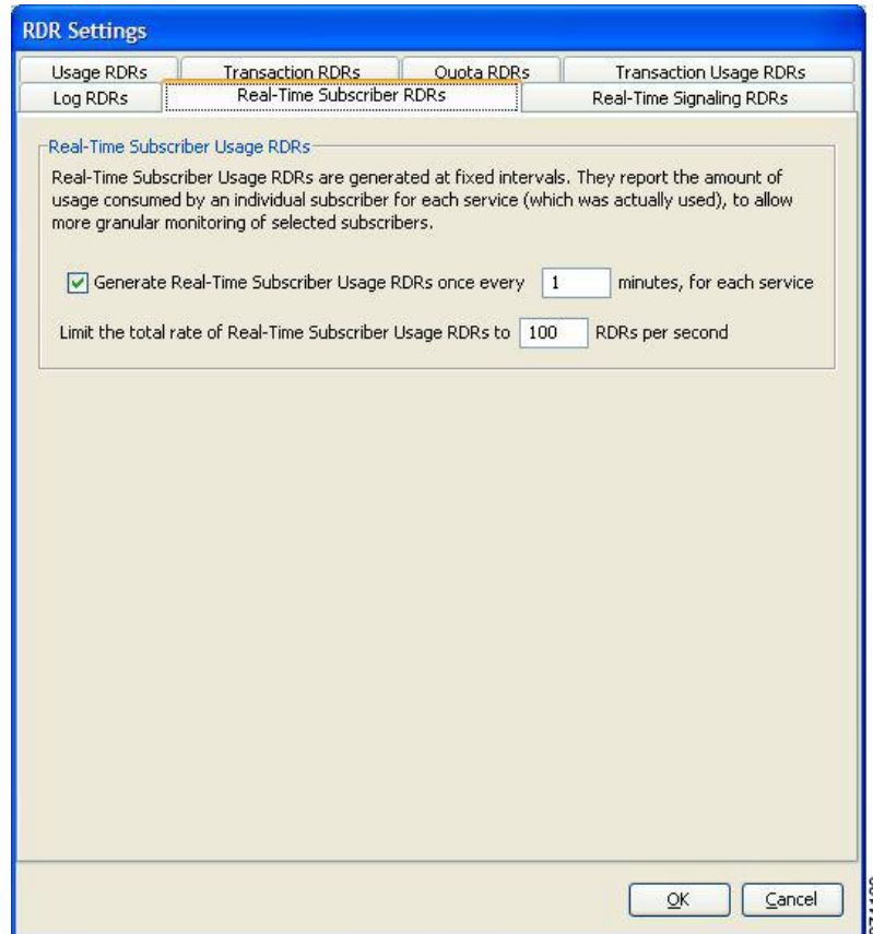
Figure 6: Real-Time Subscriber RDRs tab
