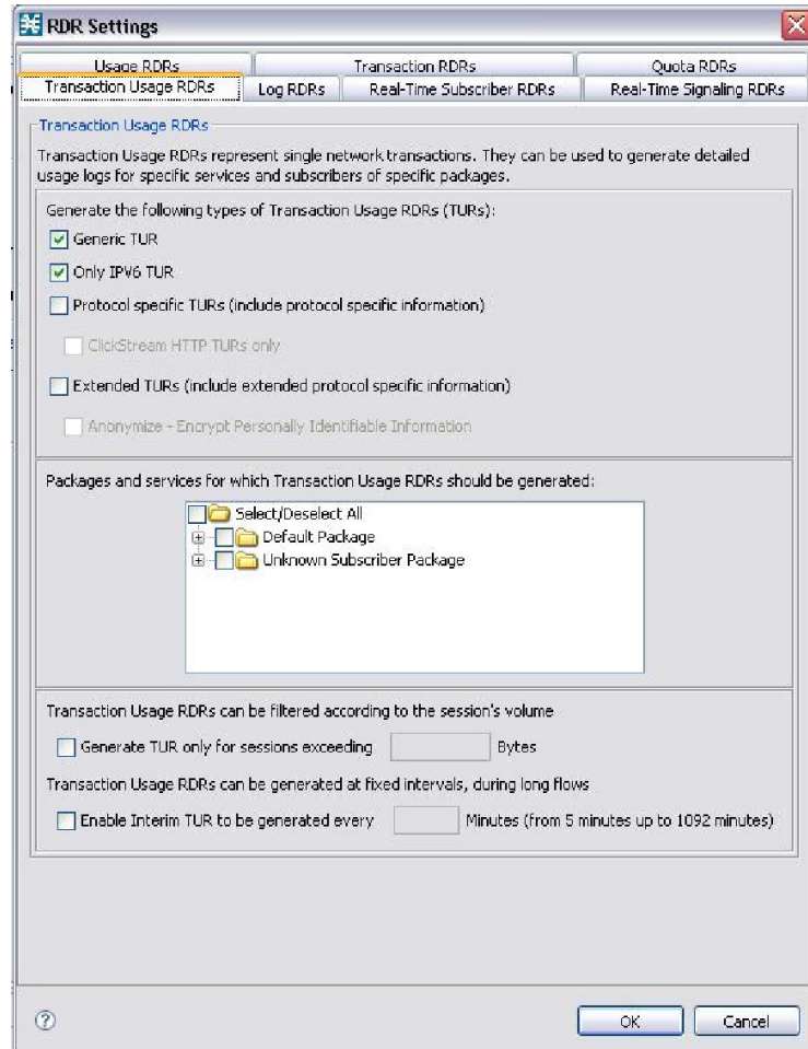
Figure 4: Transaction Usage RDRs Tab
