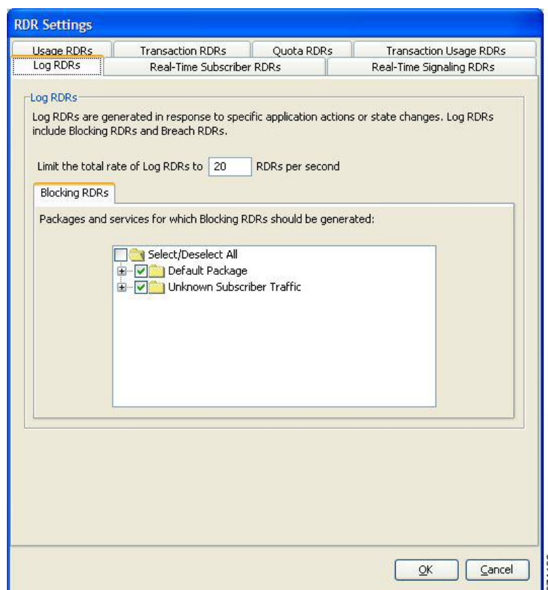
Figure 5: Log RDRs Tab
