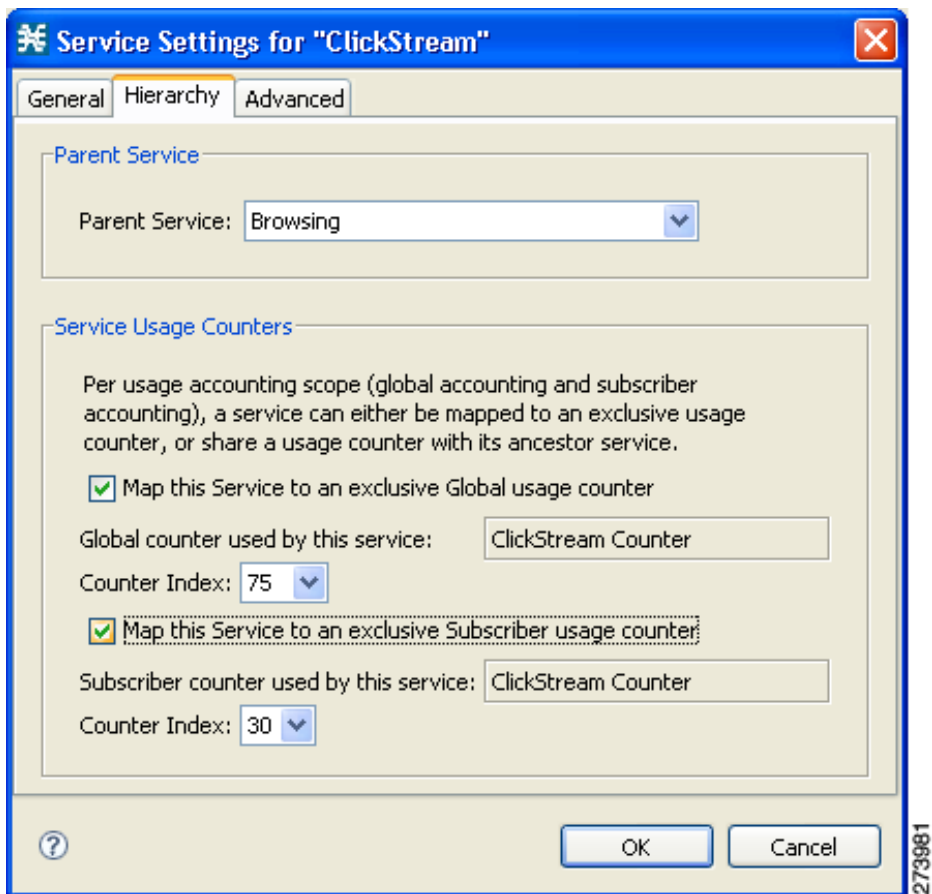
Figure 9 Hierarchy Tab
