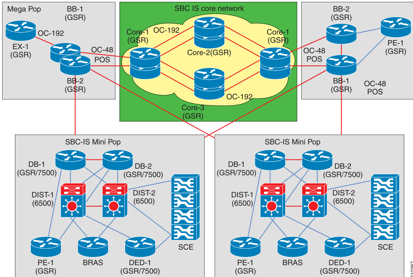
Figure 12-4 Multiple ISG Routers with Multiple SCE Platforms via Load Balancing
