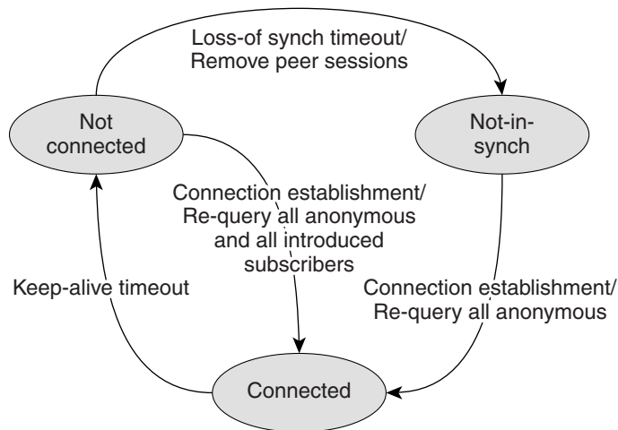
Figure 12-5 SCMP Connection State Functionality
