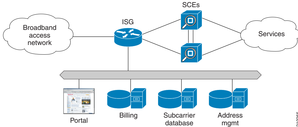
Figure 12-2 Single ISG Router with Two Cascaded SCE Platforms
