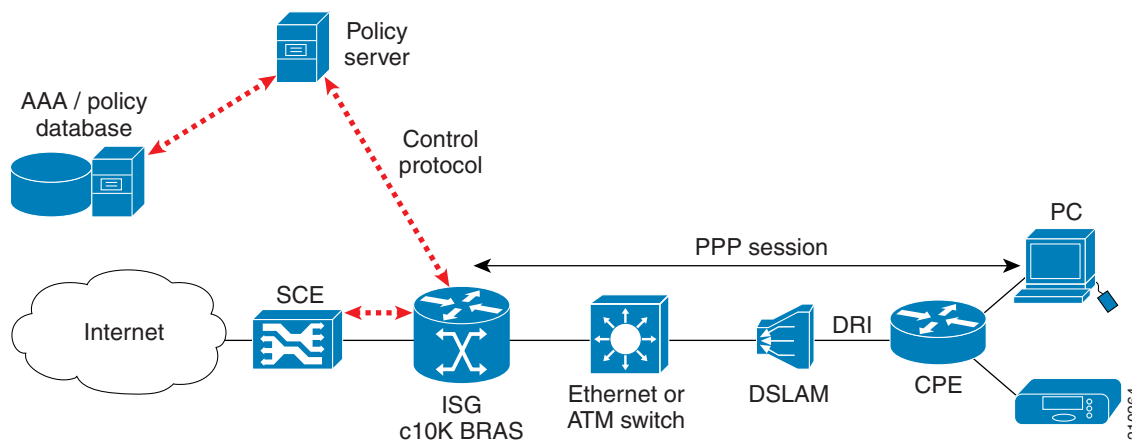
Figure 12-1 Single ISG Router with a Single SCE Platform
