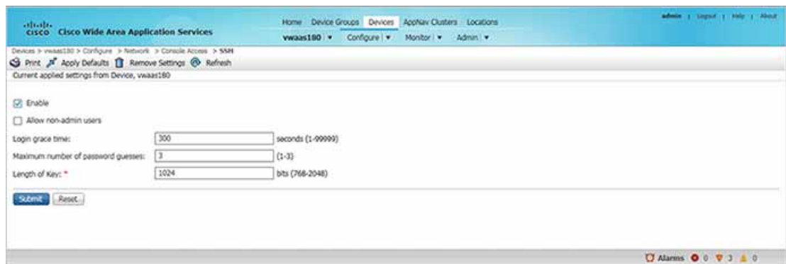
Figure 7-2 SSH Configuration Window
