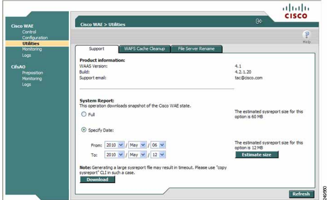
Figure 11-8 Utilities—Support Tab
